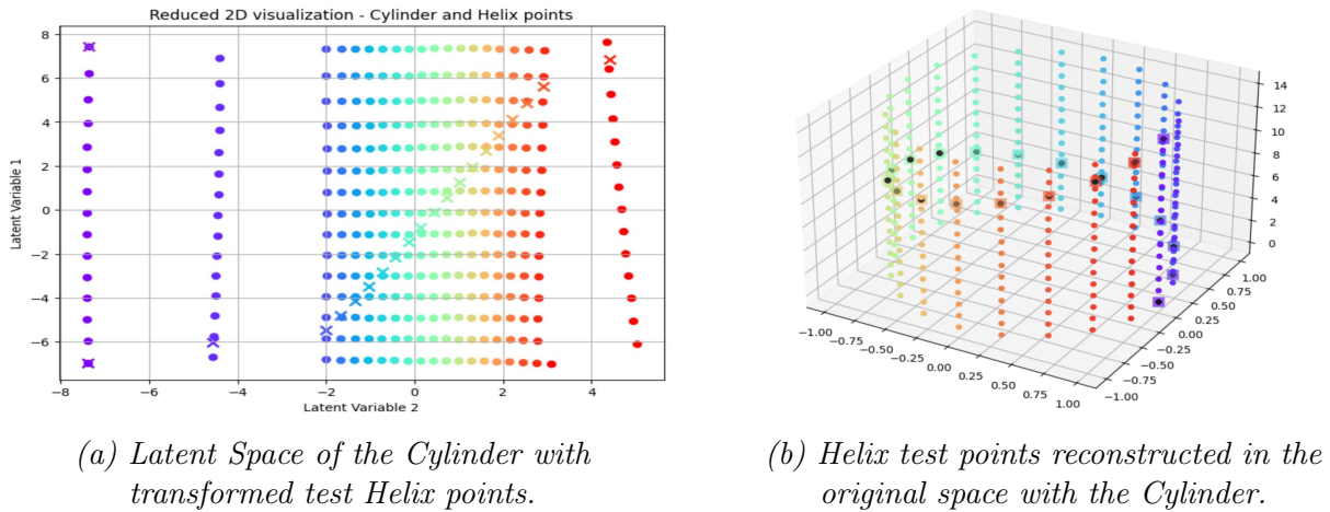
Figure 4.5: Best model, Log-Likelihood = 6475
