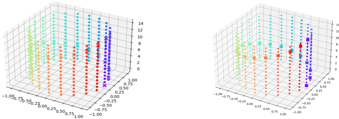
Figure 4.6: Original Helix test dataset (left) and its reconstruction with GPLVMs (right).
