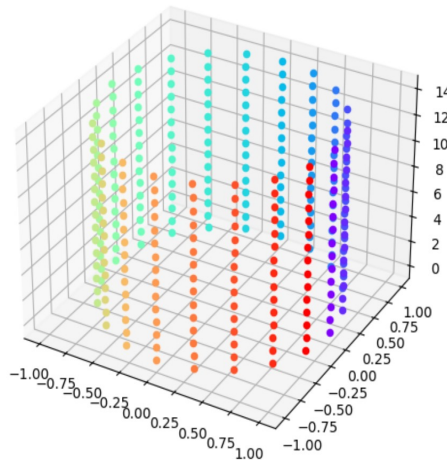
Figure 3.1: The Simulated Cylinder dataset in the observed 3-dimensional space.
