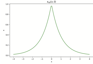
Exponential kernel
