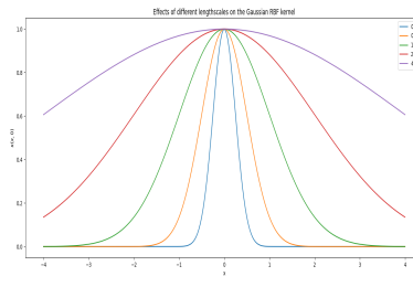
Figure 2.4: Effects of different length-scales on the Gaussian RBF kernel.
