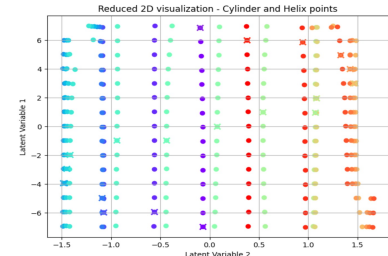
Latent space obtained
