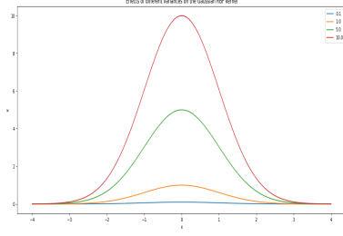
Figure 2.3: Effects of different variances on the Gaussian RBF kernel.
