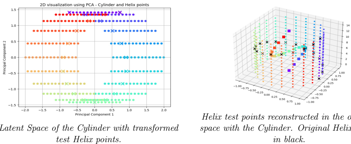
Figure 4.3: Useful plots in order to evaluate the performances of the PCA in the process of dimensionality reduction, using the Helix test dataset presented in section 3.2.
