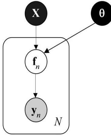
Figure 2.7: The Gaussian Process Latent Variable Model. Y is the observational space, X is the latent space and \theta are the hyperparameters of the mapping function f [Lawrence and Hyvärinen (2005)].
