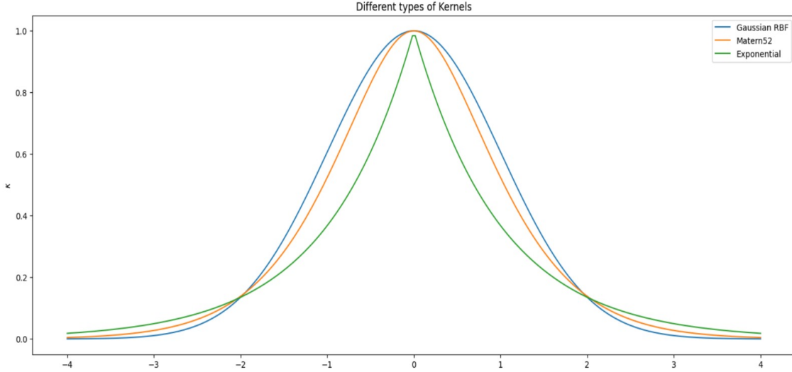
Figure 2.2: Kernel function of the three discussed kernels
